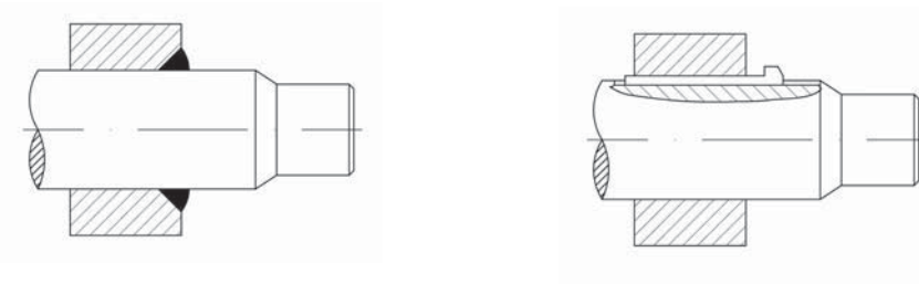
d -Smooth or tapered cotter pin
